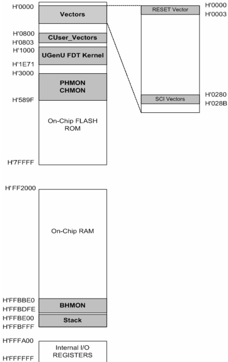
Figure 10.1: Memory Map
