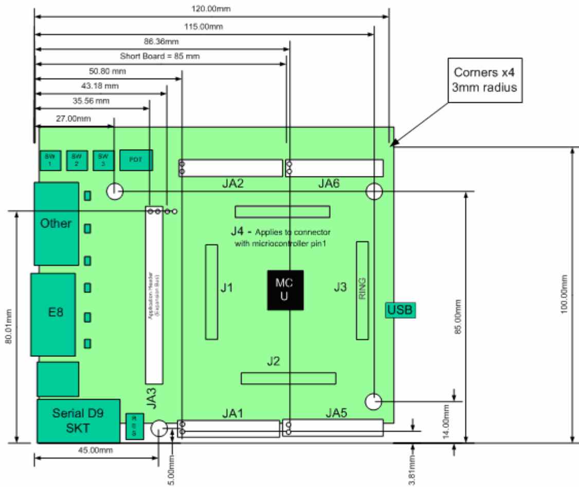
Figure 4.2 : Board Dimensions
